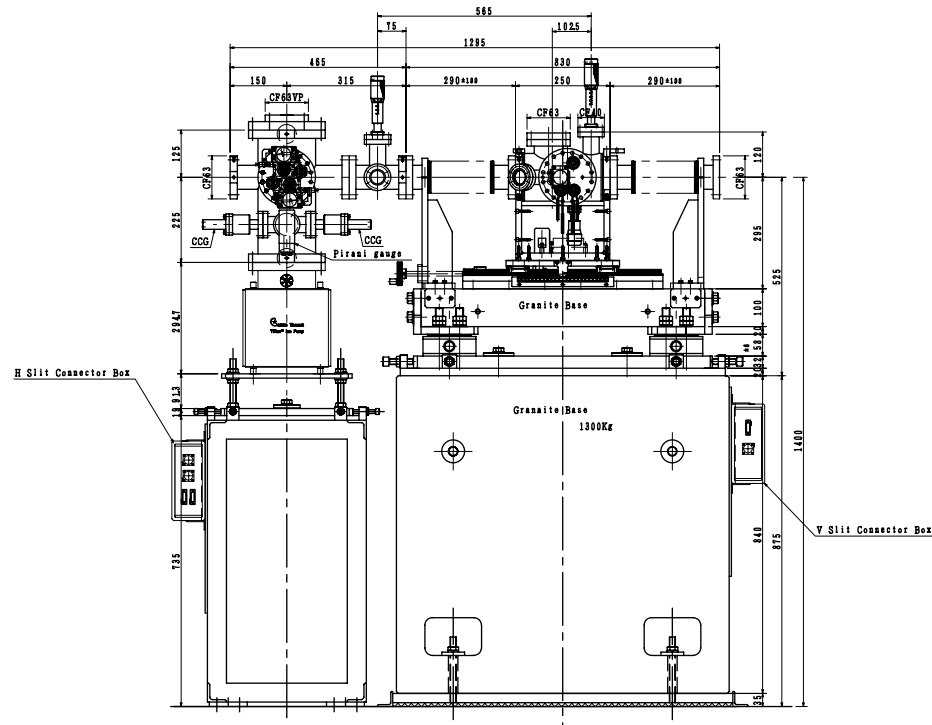
Entrance slit assembly of BOREAS beamline
